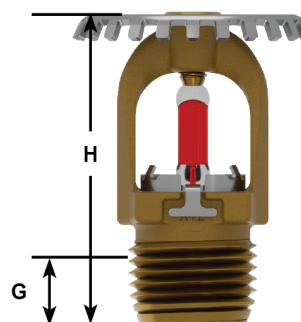
Figure – 2: Dimensions
